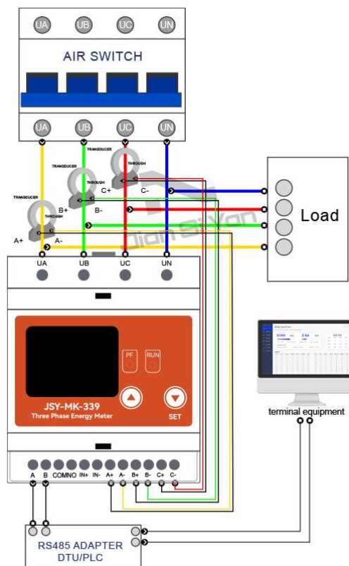
Image 4 Three-phase four-wire wiring example
