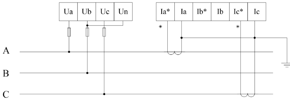
Image 3 Three-phase three-wire voltage and current connection method
