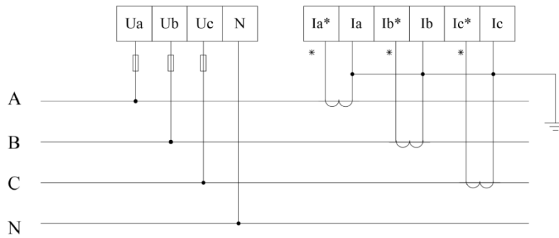
Image 2 Three-phase four-wire voltage and current connection method
