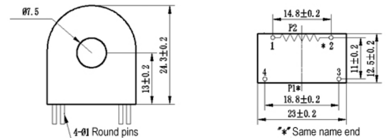
Figure 2.1 Product appearance diagram
