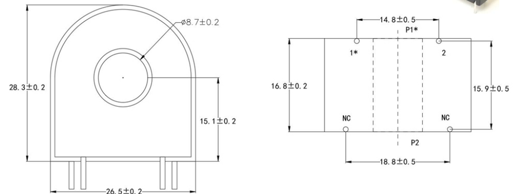
Dimensional drawing of 50A core-type current transformer
