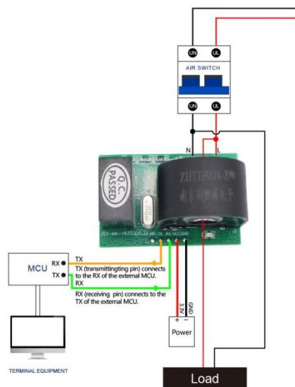
Wiring diagram
