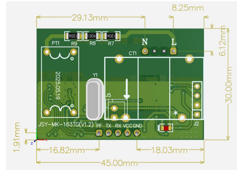
Figure 2.1 Dimensional drawing (unit: mm)
