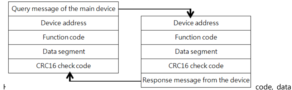
Modbus protocol query response data flow
