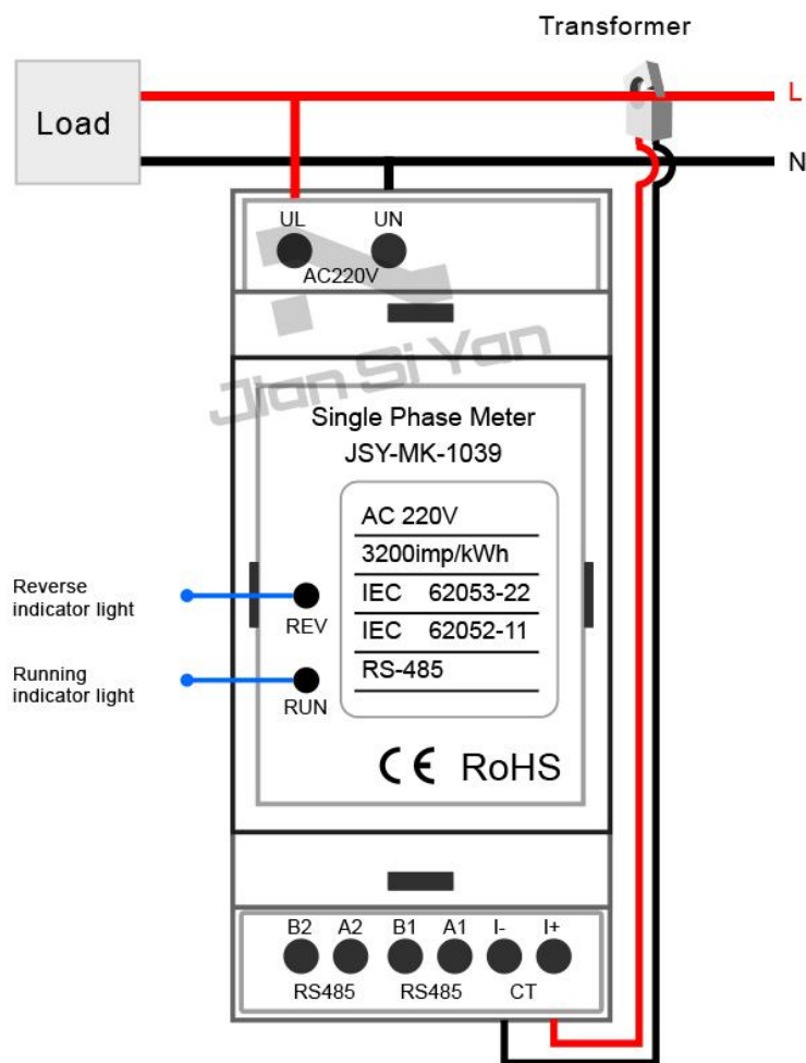
Wiring Diagram
